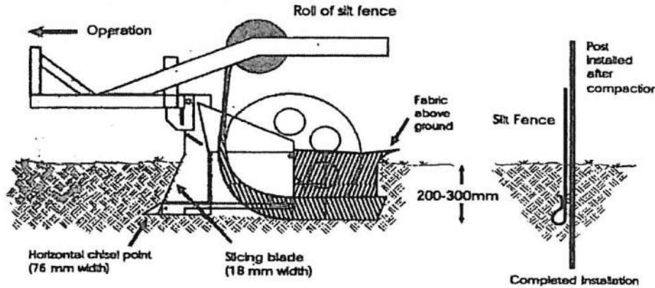
Vibratory plow is not acceptable because of horizontal compaction
